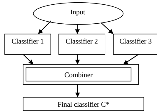
Fig.2 Ensemble Learning
