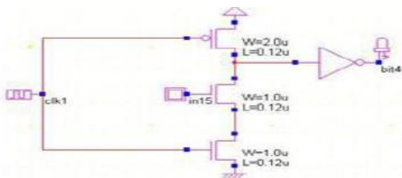
Fig.7. Bit4 of a 5-Bit Dynamic Thermometer Encoder.
