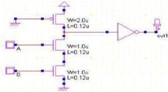
Fig.2. Schematic of Two Input AND Gate using Pseudo NMOS Logic.
