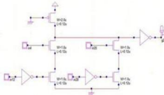
Fig.4. Schematic of 2 Input XOR Gate using pseudo Dynamic Logic.
