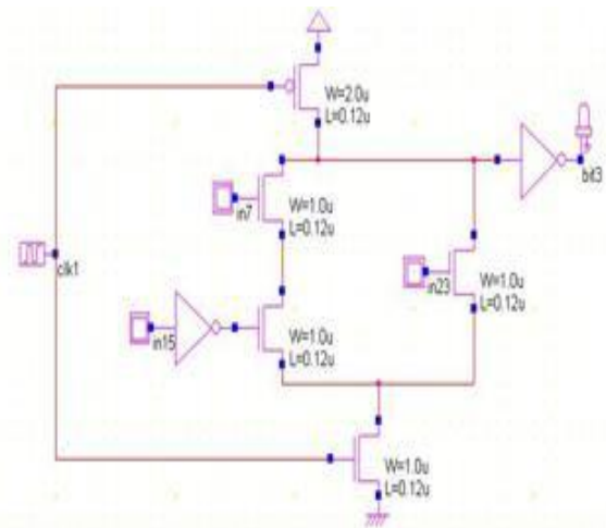
Fig.8. Bit3 of a 5-Bit Dynamic Thermometer Encoder.
