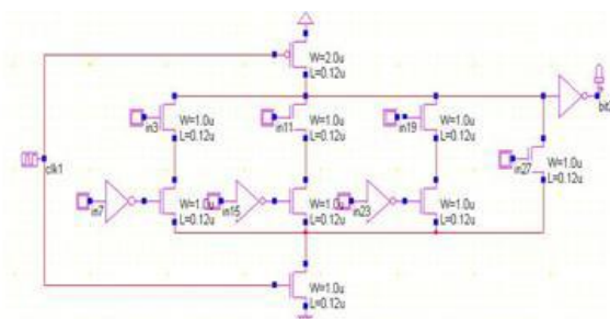
Fig.9. Bit2 of a 5-Bit Dynamic Thermometer Encoder.
