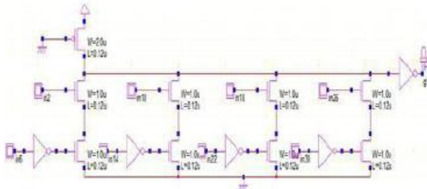
(b) Gray Code Bit1 Generation Circuit
