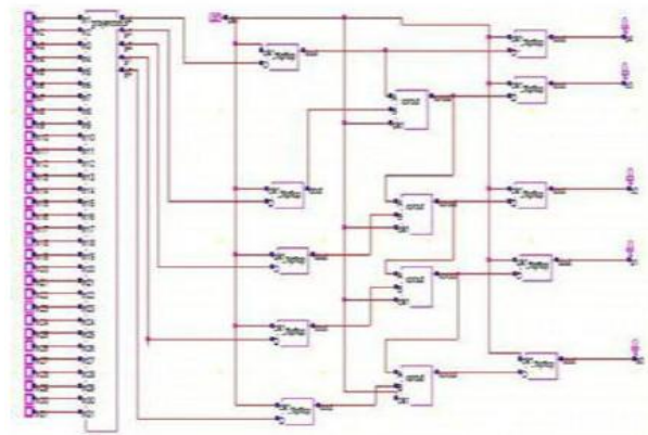
Fig.6. Gray Code to Binary Code Encoder
