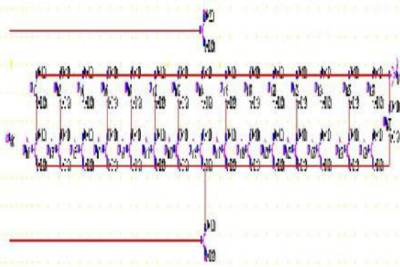
Fig.11. Bit0 of a 5-Bit Dynamic Thermometer Encoder.
