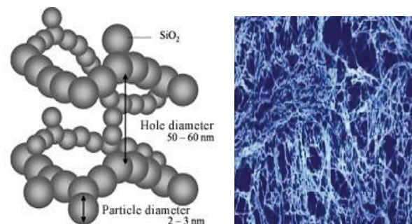
Fig. 1 : Nanometer-scale particles and pores in an aerogel. (a) Network architecture of an aerogel [15]. (b) Electron micrograph of a silica aerogel [2].
