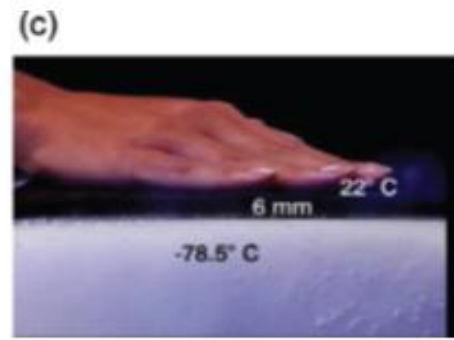
Fig.5 : Flexible aerogel blankets and solid aerogel boards. (a) Aerogel blankets (b) aerogel panel and (c) super insulating aerogel blanket
