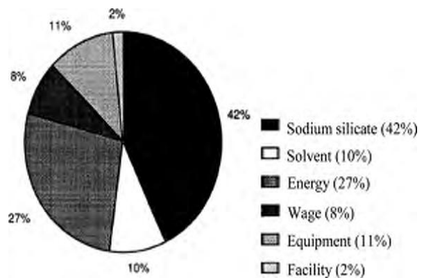
Fig. 7 : Aerogel cost distribution (sodium silicate) [32].
