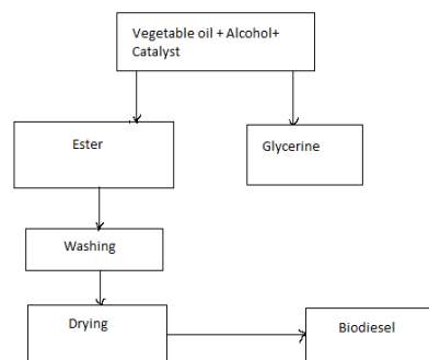
Fig.1 Biodiesel Production
