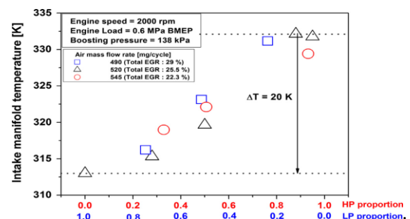
Fig.10 Intake manifold temperature Vs HP/LP EGR proportion [9]
