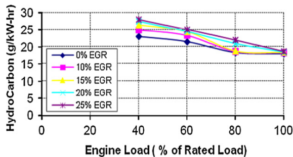
Fig.6 Hydrocarbons for different EGR rates [4]
