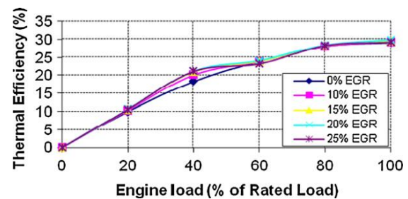
Fig.3 Thermal Efficiency for Different EGR Rate [4]
