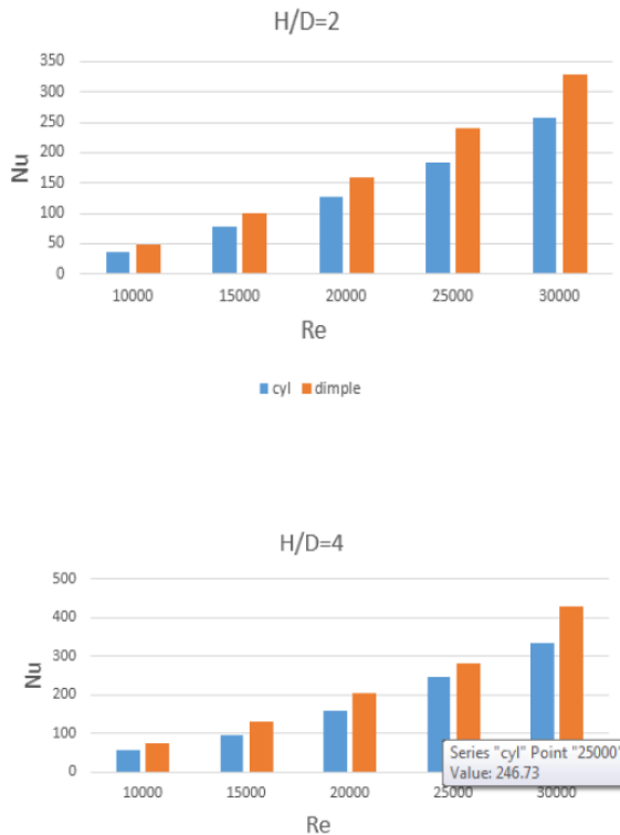
Figure 2 Variation of Nu Vs Re at H/D=2 and H/D=4
