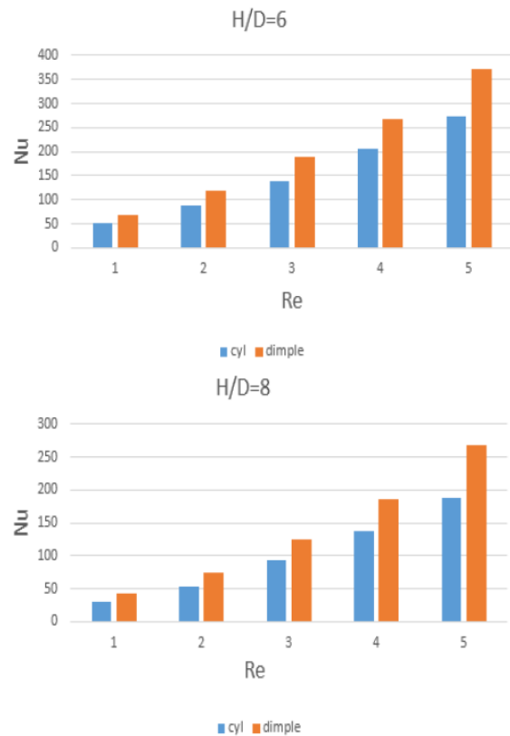
Figure 3 Variation of Nu Vs Re at H/D=6 and H/D=8
