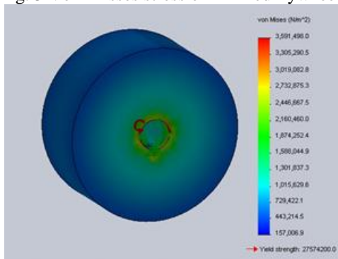
Fig. 4 Von-Misses stress on solid disc flywheel
