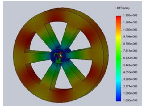
Fig. 6 Analysis of Displacement in solid disc flywheel.
