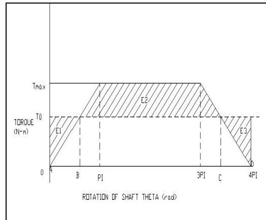
Fig.1 T-θ diagram
