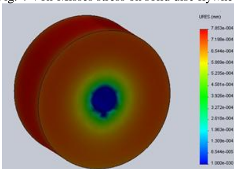
Fig.5 Analysis of Displacement in rimmed flywheel.
