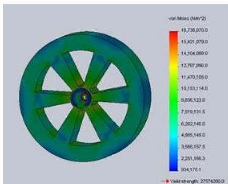
Fig. 3 Von-Misses stress on rimmed flywheel.
